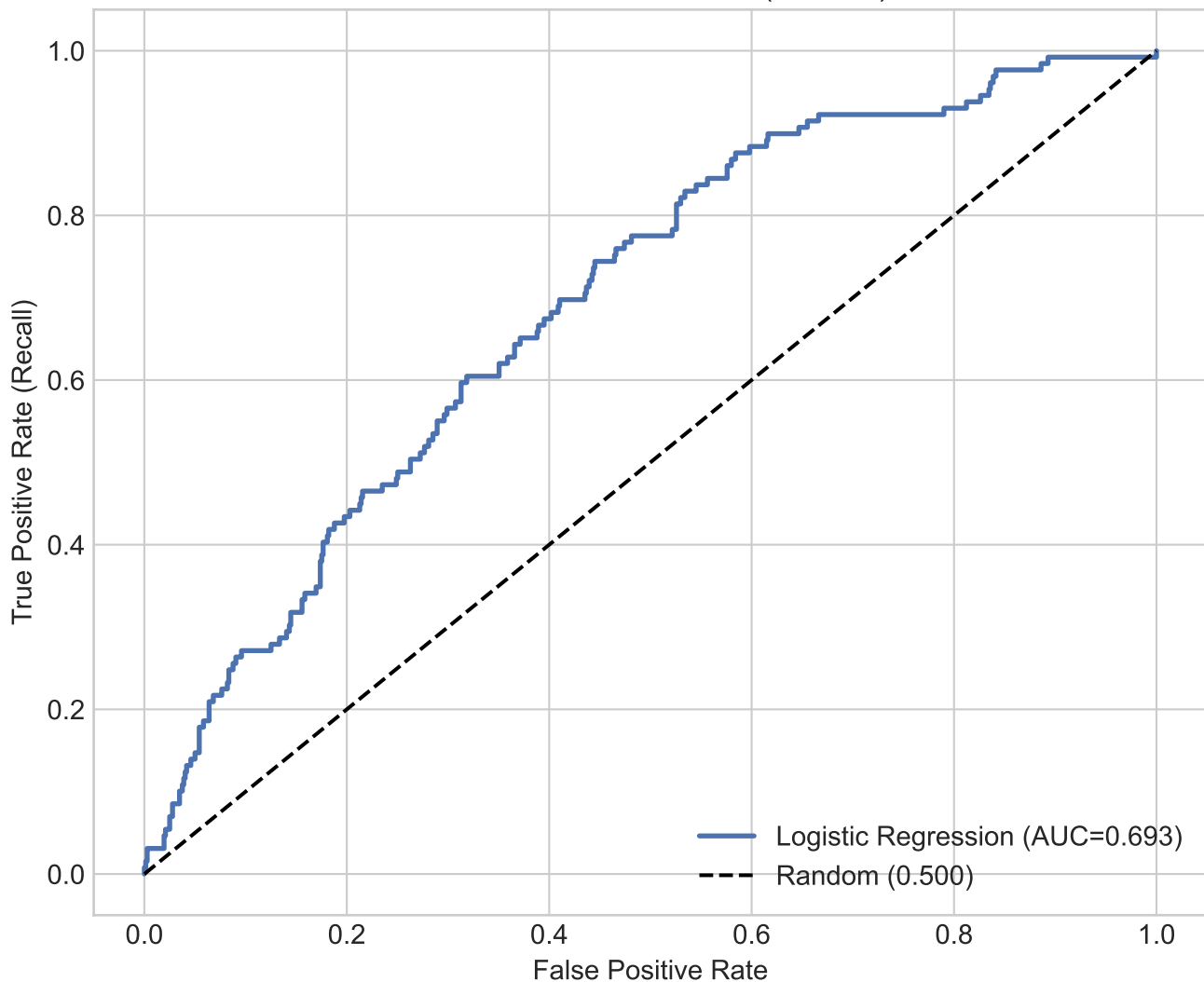
Final model ROC curve (test set)
